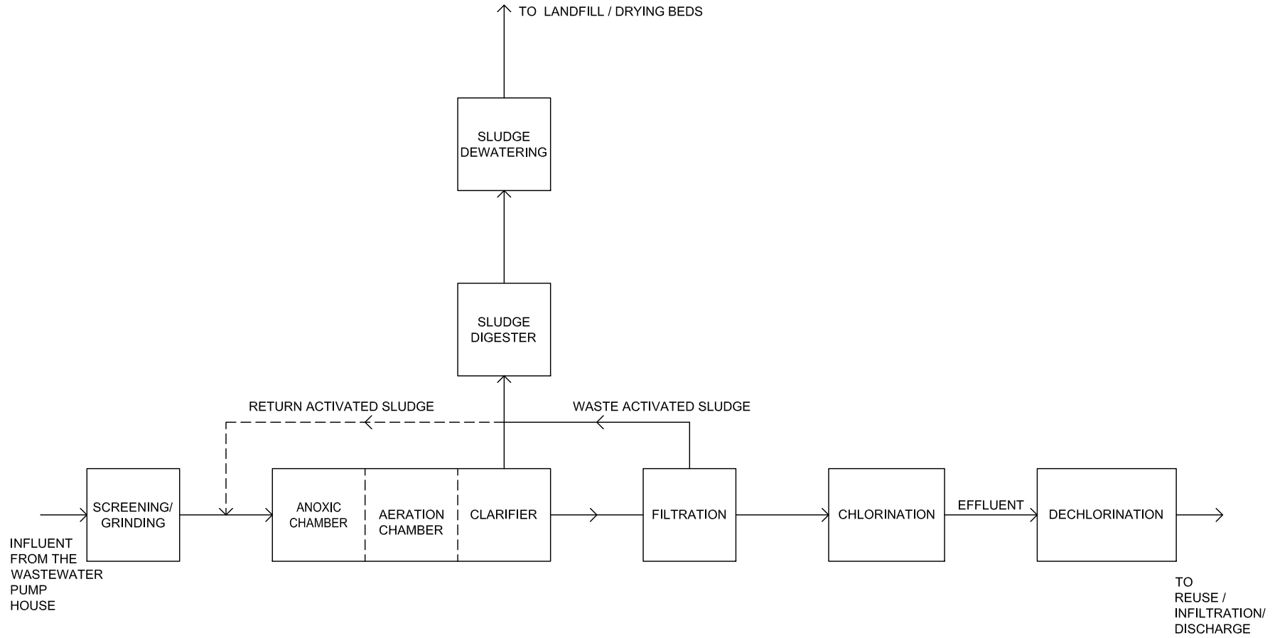
FIGURE 7 CONCEPTUAL PROCESS FLOW DIAGRAM DRAFT CAAG 208 PLAN AMENDMENT - MIAMI WASTEWATER RECLAMATION FACILITY
